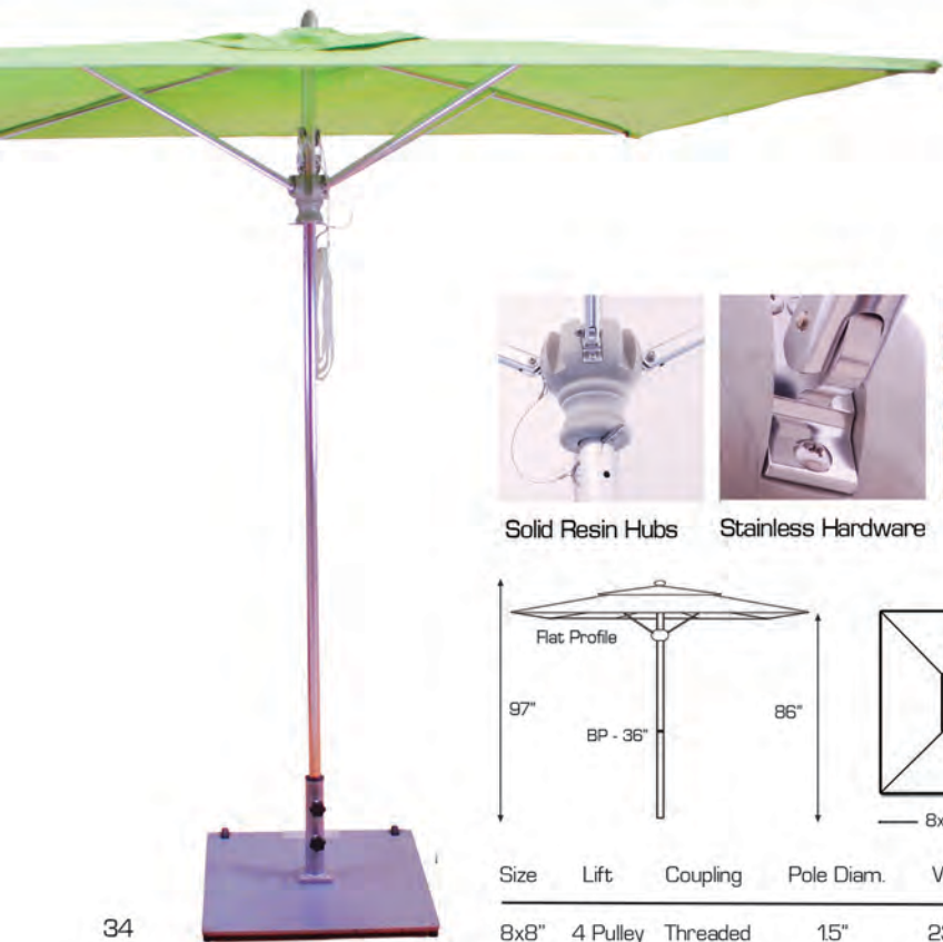
Threaded Coupling
